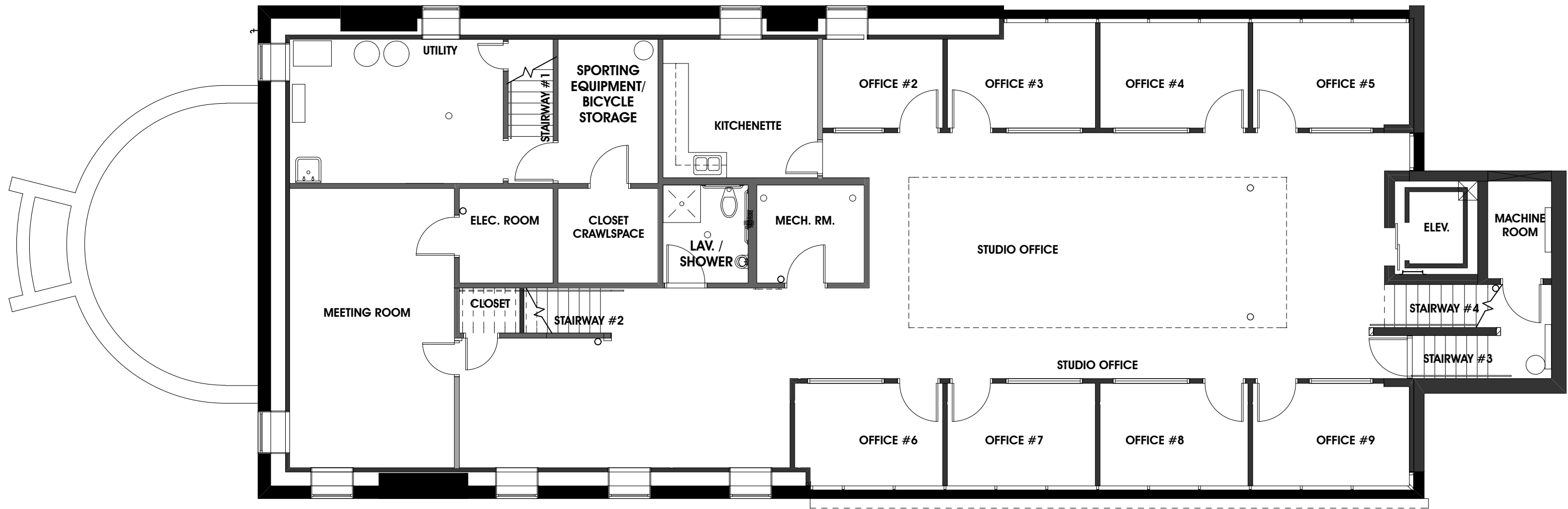
FLOOR PLAN BASEMENT LEVEL SCALE: 1'-0" = 3/32"
